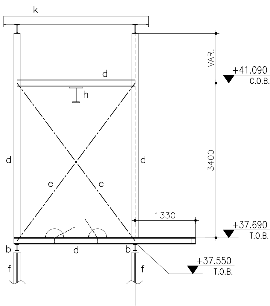
VIEW "C1" SC. 1:50
