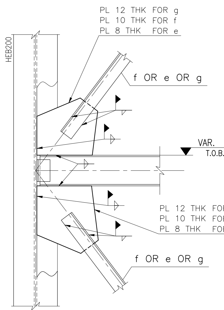
TYPICAL SEC. OF VER. BRACING SEE SCHEDULE-1&2(SS002) SC. 1:10
