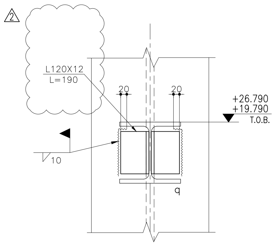
SEC. 2-2 SC. 1:10
