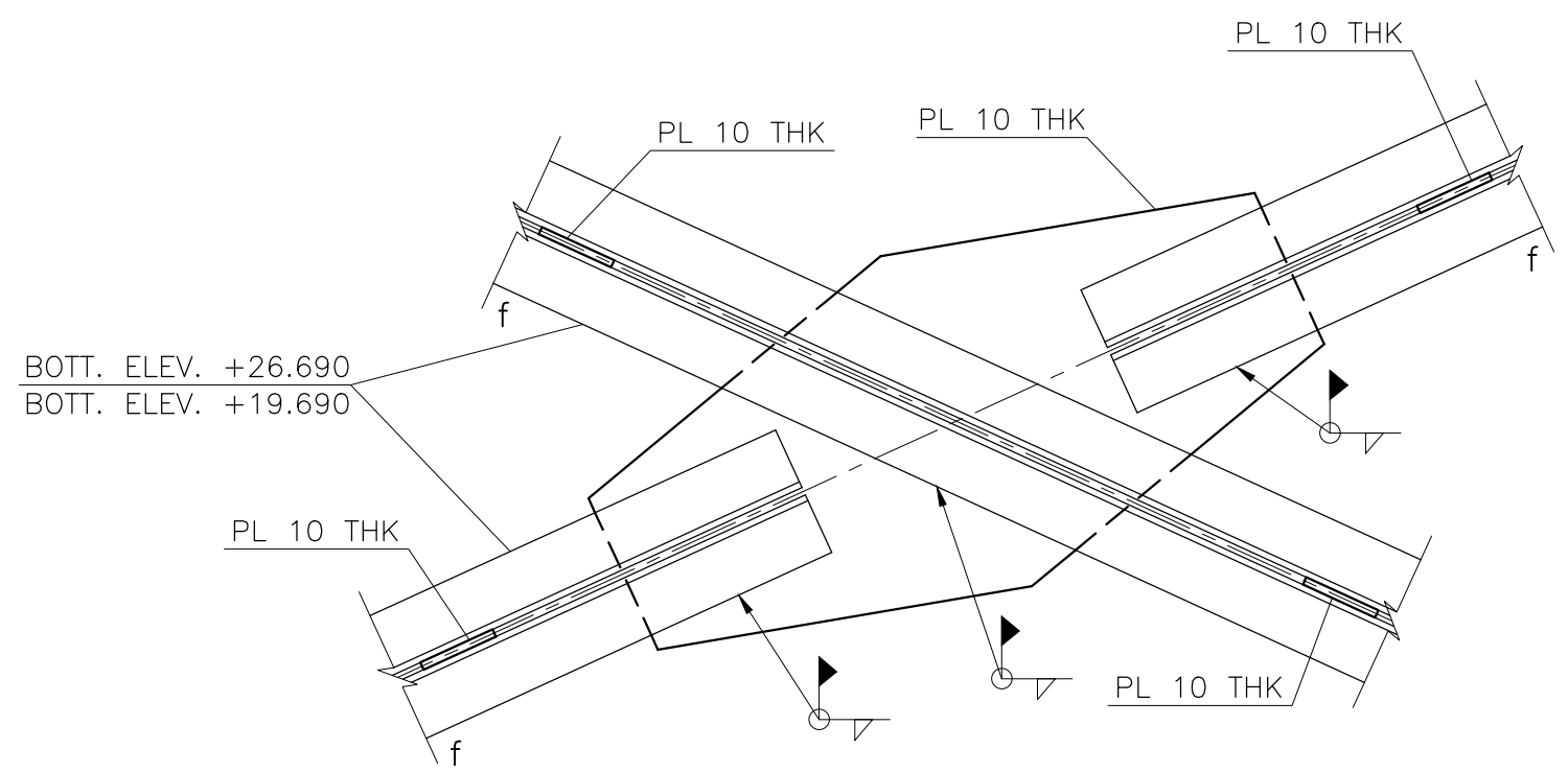
DET. "12" SS005 SC. 1:10 SS007 SEE SCHEDULE-1&2(SS002)
