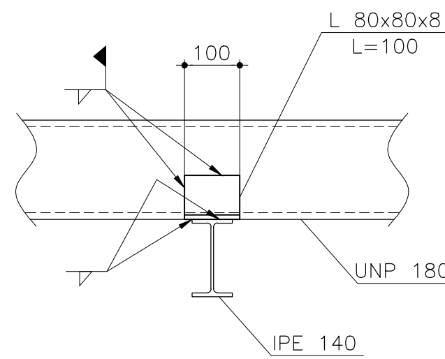
SEC. 1-1 Sc. 1:10
