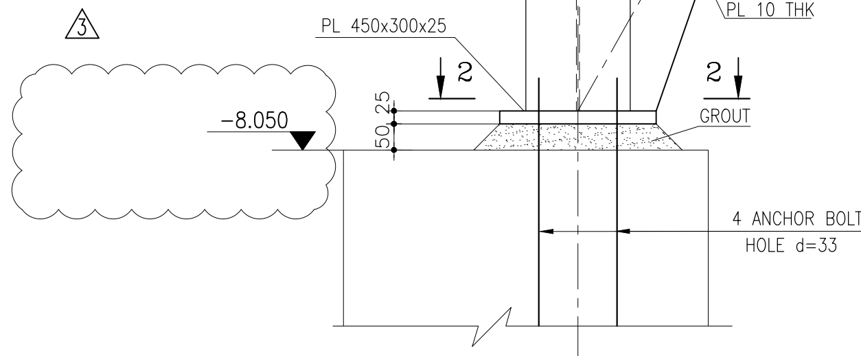
DET. "23" SS012 SC. 1:10 SEE SCHEDULE-1&2(SS002)
