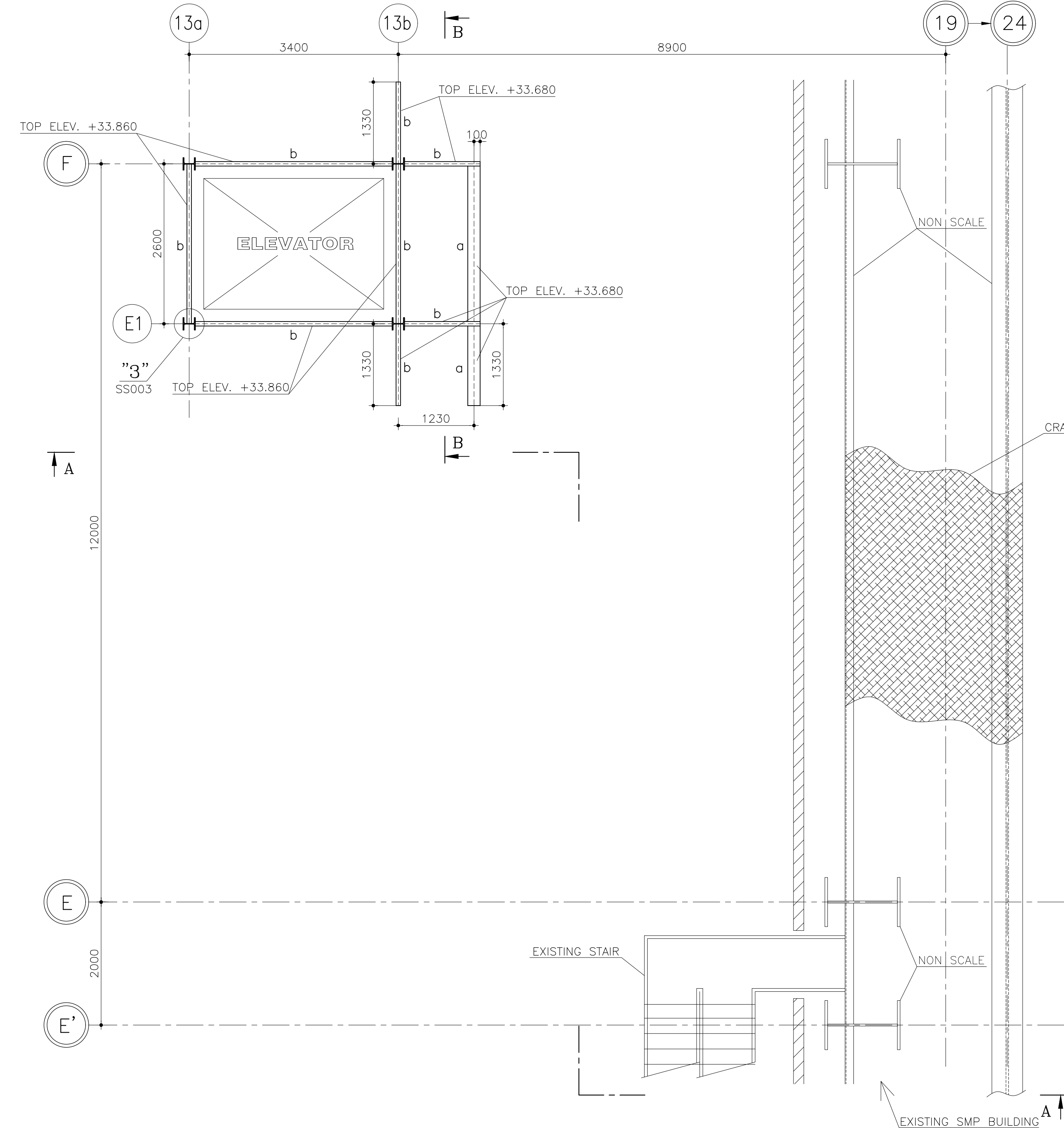
BEAMS PLAN AT ELEV. +33.680 & +33.860 ALL ELEVATION=T.O.B. SC. 1:50
