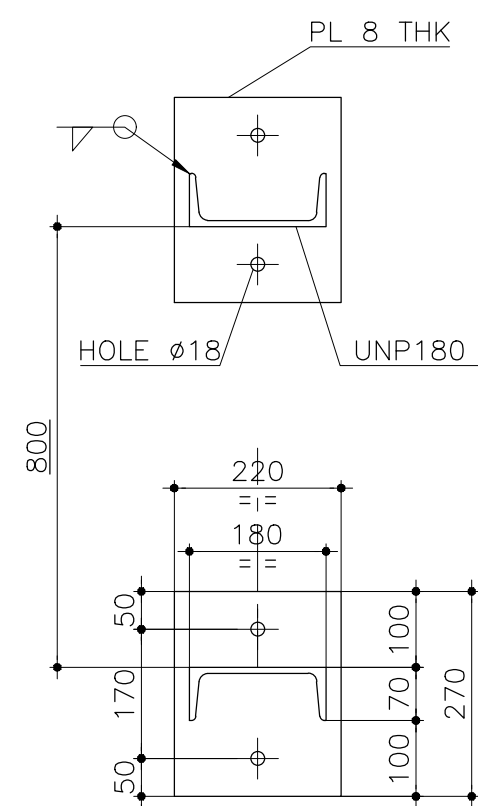
SEC. 1-1 SC. 1:10
