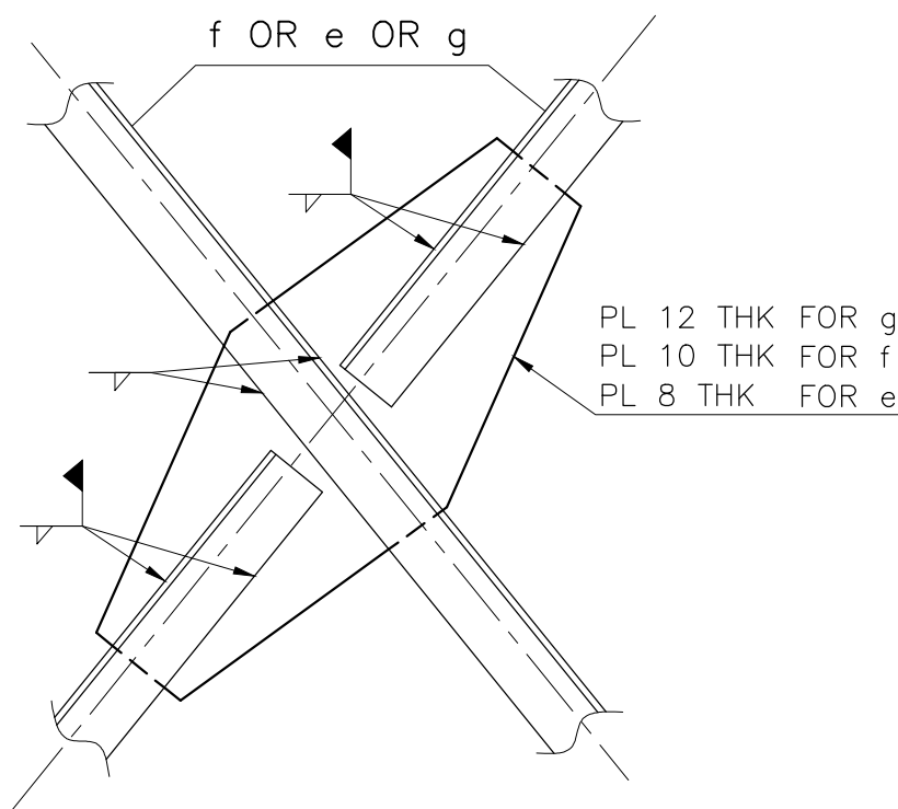
TYPICAL SEC. OF VER. BRACING SEE SCHEDULE-1&2(SS002) SC. 1:10
