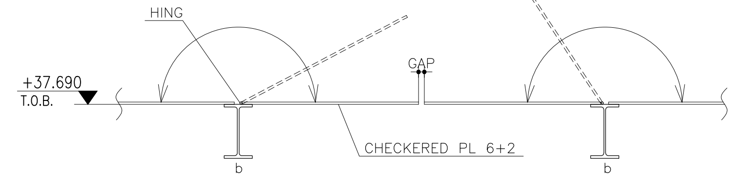
SEC. 2-2 SC. 1:10
