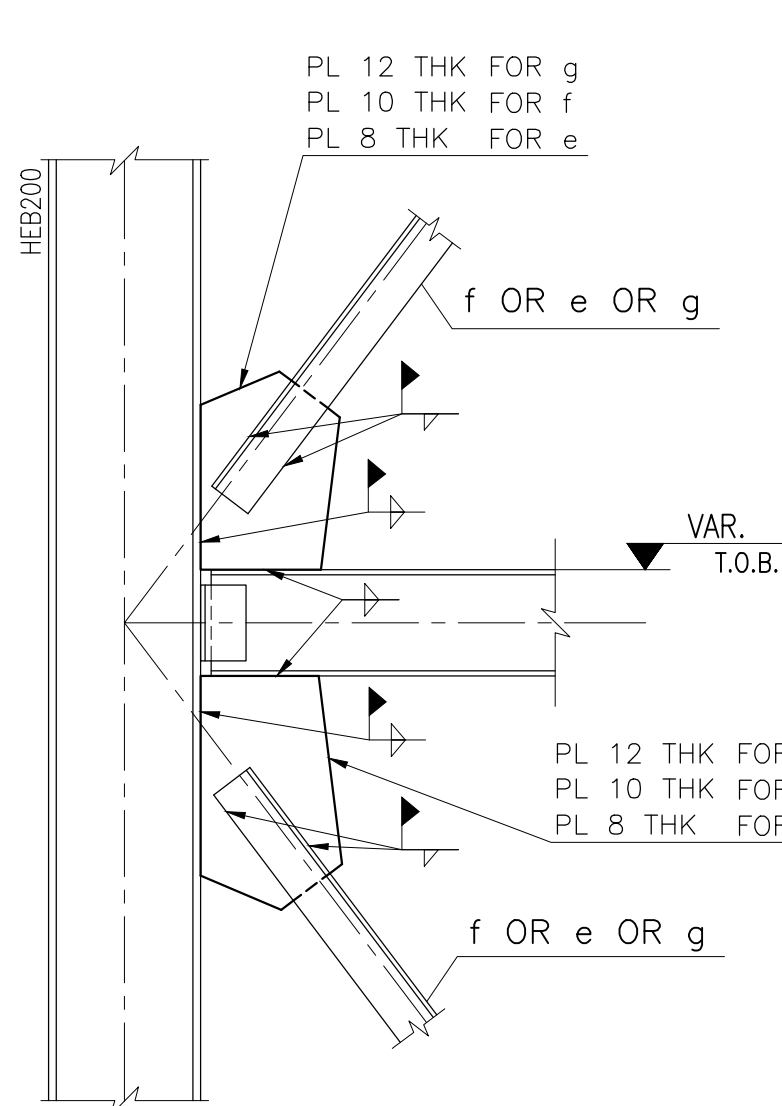
TYPICAL SEC. OF VER. BRACING SEE SCHEDULE-1&2(SS002) SC. 1:10
