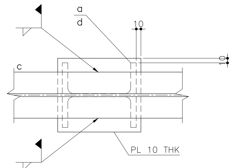
SEC. 7-7 & 8-8 Sc. 1:5
